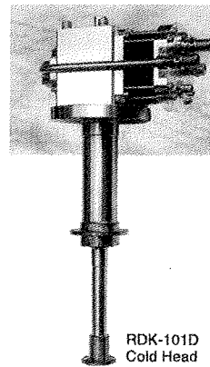
Fig. 13. Two-stage cold head and compressor for small 4-K GM refrigerator. Courtesy Sumitomo Heavy Industries.
