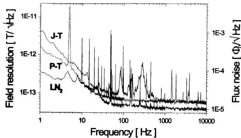
Fig. 21. Field noise in a SQUID caused by various cooling methods. Reproduced from [43] by permission of IEEE.
