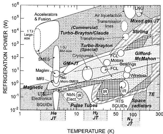
Fig. 18. Application map of cryocoolers as shown in Fig. 1 (clear regions) superimposed on typical operating regions (crosshatched) for various types of cryocoolers.
