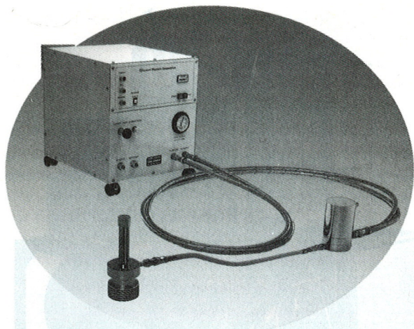
Fig. 14. Commercial pulse tube refrigerator with rotary valve and GM compressor. Courtesy Iwatani.
