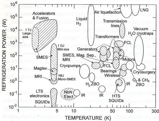
Fig. 1. Map of cryocooler applications in plane of refrigeration power versus temperature. Superconductivity applications are shown as crosshatched regions.
