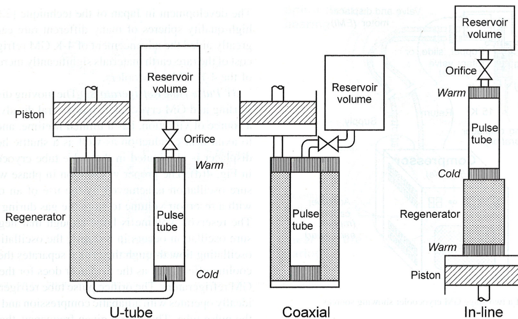
Fig. 9. Three different geometries for pulse tube refrigerators.
