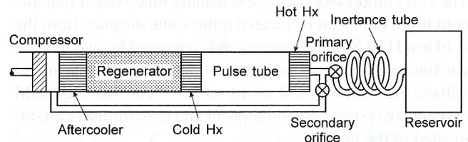
Fig. 10. Schematic of pulse tube refrigerator with secondary orifice (double inlet) and inertance tube.
