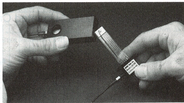
Fig. 5. Open-cycle JT cryocooler with gas channels etched in glass. Courtesy MMR.
