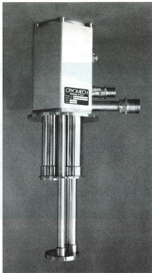
Fig. 15. Commercial two-stage pulse tube refrigerator for temperatures down to 4 K. Courtesy Cryomech.
