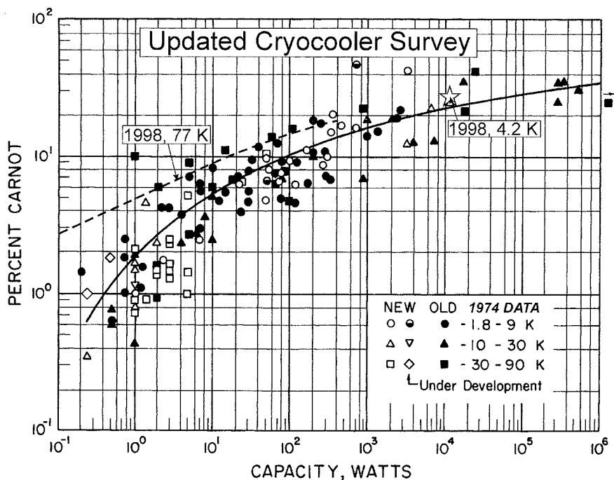
Fig. 3. Second-law efficiency of cryocoolers as a function of refrigeration power.
