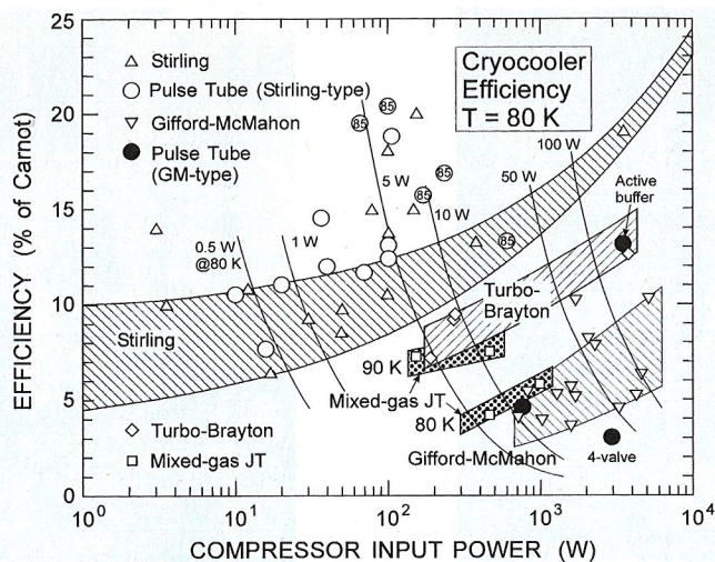
Fig. 19. Efficiencies of various types of cryocoolers at 80 K.
