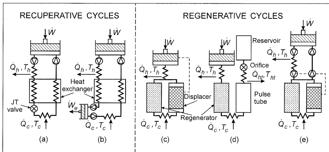
Fig. 4. Schematics of five common types of cryocoolers.
