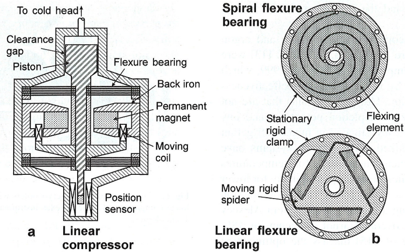
Fig. 7. Schematic of: (a) linear compressor with flexure bearings and (b) two types of flexure bearings.
