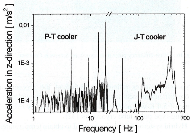
Fig. 20. Vibration at cold tip of pulse tube and mixed-gas JT cryocoolers. Reproduced from [43] by permission of IEEE.
