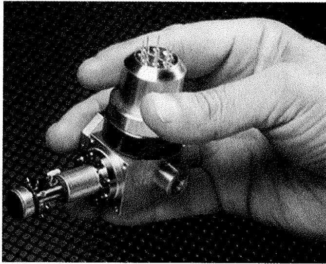
Fig. 11. Photos of miniature and large Stirling refrigerators. Courtesy FLIR/Inframetrics and Stirling Cryogenics & Refrigeration.
