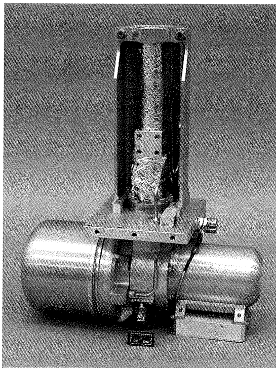
Fig. 16. High-efficiency pulse tube cryocooler for space. Courtesy TRW.
