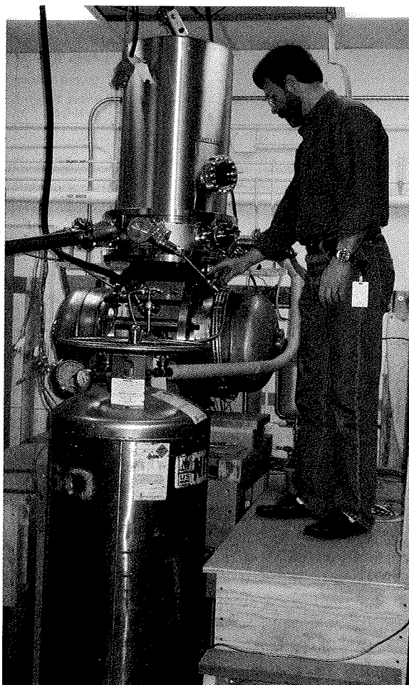
Fig. 17. Large pulse tube neon liquefier with 20-kW flexure bearing compressor.
