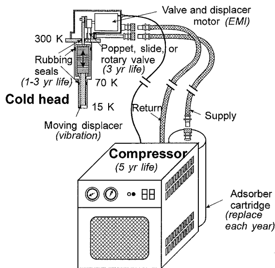
Fig. 8. Drawing of a two-stage GM cryocooler showing sources of concern to users.
