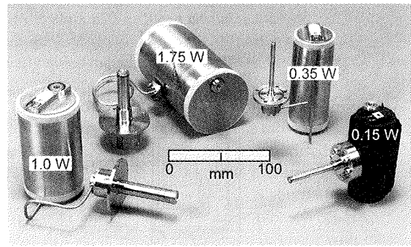
Fig. 6. Four sizes of Stirling cryocoolers with dual-opposed linear compressors. Courtesy Texas Instruments/DRS Infrared Technologies.
