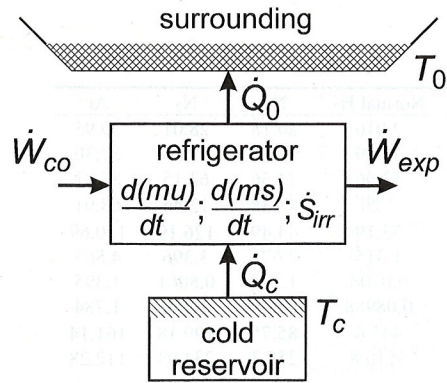
Fig. 2. Schematic of a refrigerator shown as a closed thermodynamic element along with the important thermodynamic parameters.
