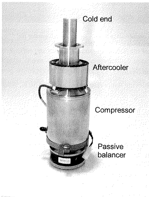
Fig. 12. Stirling cryocooler used for cooling HTS microwave filters in cellular phone base stations. Courtesy STI.
