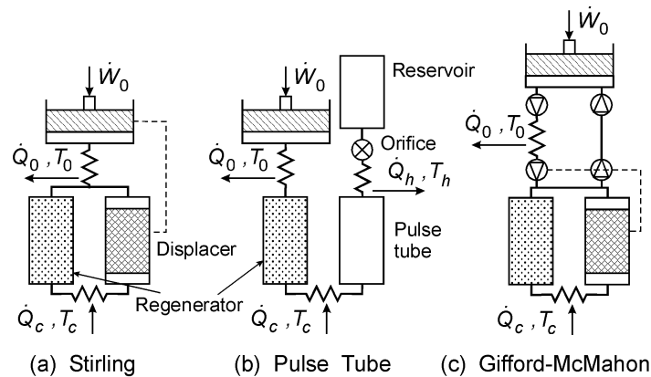
Figure 2. Schematics of regenerative cryocoolers
