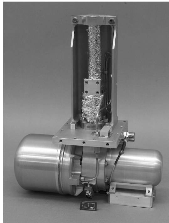
Figure 12. High efficiency pulse tube refrigerator
