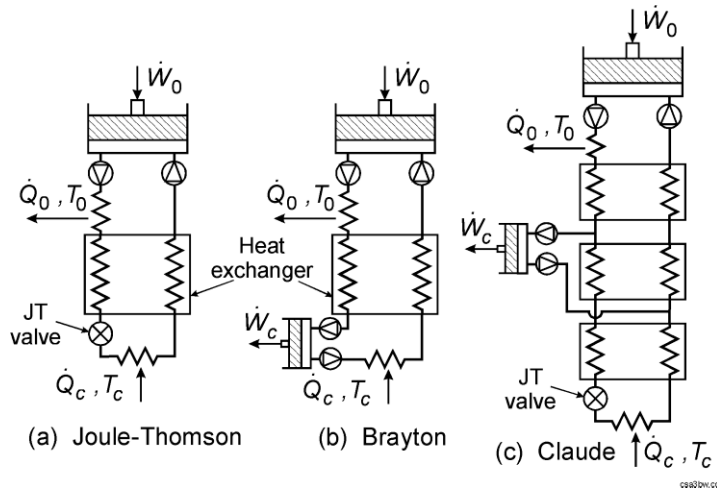
Figure 1. Schematics of recuperative cryocoolers
