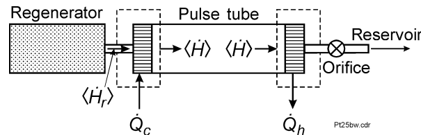
Figure 3. First law energy balance
