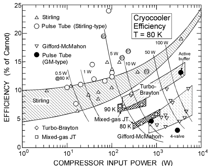
Figure 8. Efficiency of various types of cryocoolers at 80 K
